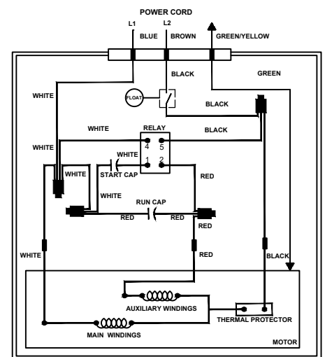
SINGLE PHASE AUTO WIRING DIAGRAM (220 V / 50 Hz)
